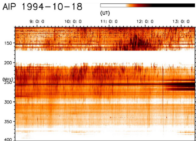
Figure 27: An example of a solar radio noise storm on 18 October 1994 as seen in a radio spectrogram (courtesy the Astrophysikalisches Institut Potsdam). The numerous short-duration, narrow-band bursts are noise storm emission and indicate continued particle acceleration.
