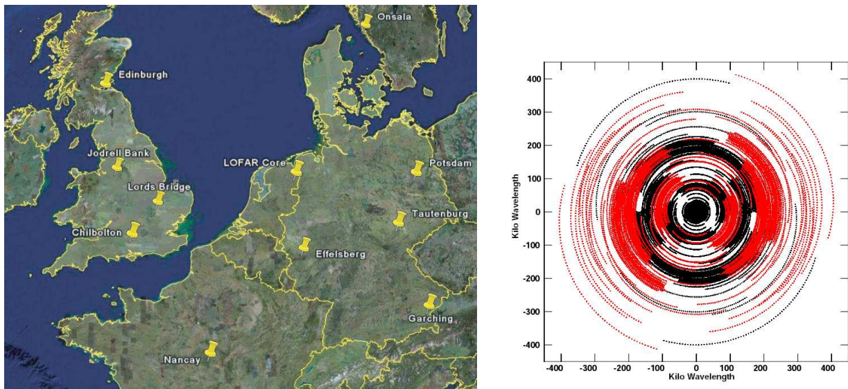
Figure 3: Left: The locations of currently funded international stations in Germany, France and Sweden, together with the proposed 4 UK stations. Right: A simulation of the (u-v) coverage (at 100 MHz) provided by the currently funded Dutch and international LOFAR stations, together with the proposed UK stations. Baselines involving UK stations are shown in red.
