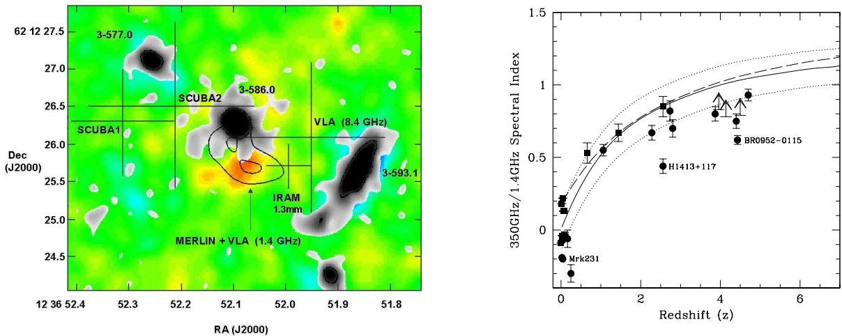
Figure 13: Left : Positional information on HDF850.1, overlaid on a K - I colour image of the field (from Dunlop et al., 2004). The SCUBA1 and SCUBA2 crosses represent position estimates from two different reductions of the SCUBA data. The positions from VLA 8.4 GHz and IRAM PdB 1.3 mm detections are also shown. In all cases the size of the cross indicates the 1\sigma error in the relevant position. The contours show a high resolution MERLIN+VLA 1.4 GHz radio map. Only with this sub-arcsec resolution was the host galaxy of HDF850.1 able to be associated with an optically faint extremely red galaxy. This demonstrates the need for international baselines to increase the angular resolution of LOFAR. Right : The modelled and observed radio to sub-mm flux ratio as a function of redshift (from Carilli & Yun, 2000). This flux ratio allows a reliable redshift estimate out to z \sim 3 .
