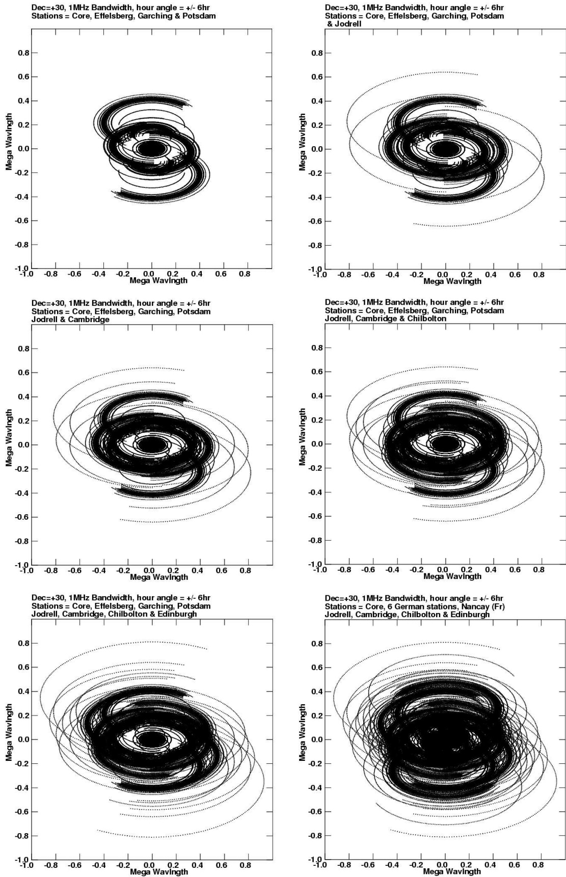
Figure 31: The simulated u-v tracks for full 12 hr (hour angle \pm 6 ) synthesis observations of a source at 30^\circ declination, at 230 MHz with 1 MHz bandwidth. The various combinations of LOFAR stations are as described in Figure 30.
