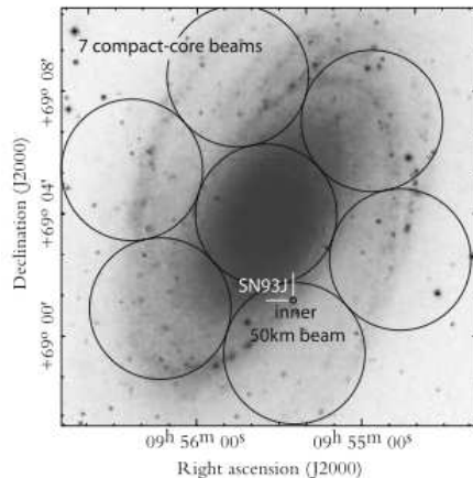
Figure 23: Coherently formed beams from the compact core and the inner 50-km of LOFAR, projected on the core of M81, the second best candidate galaxy for an extragalactic survey and the home of supernova 1993J.
