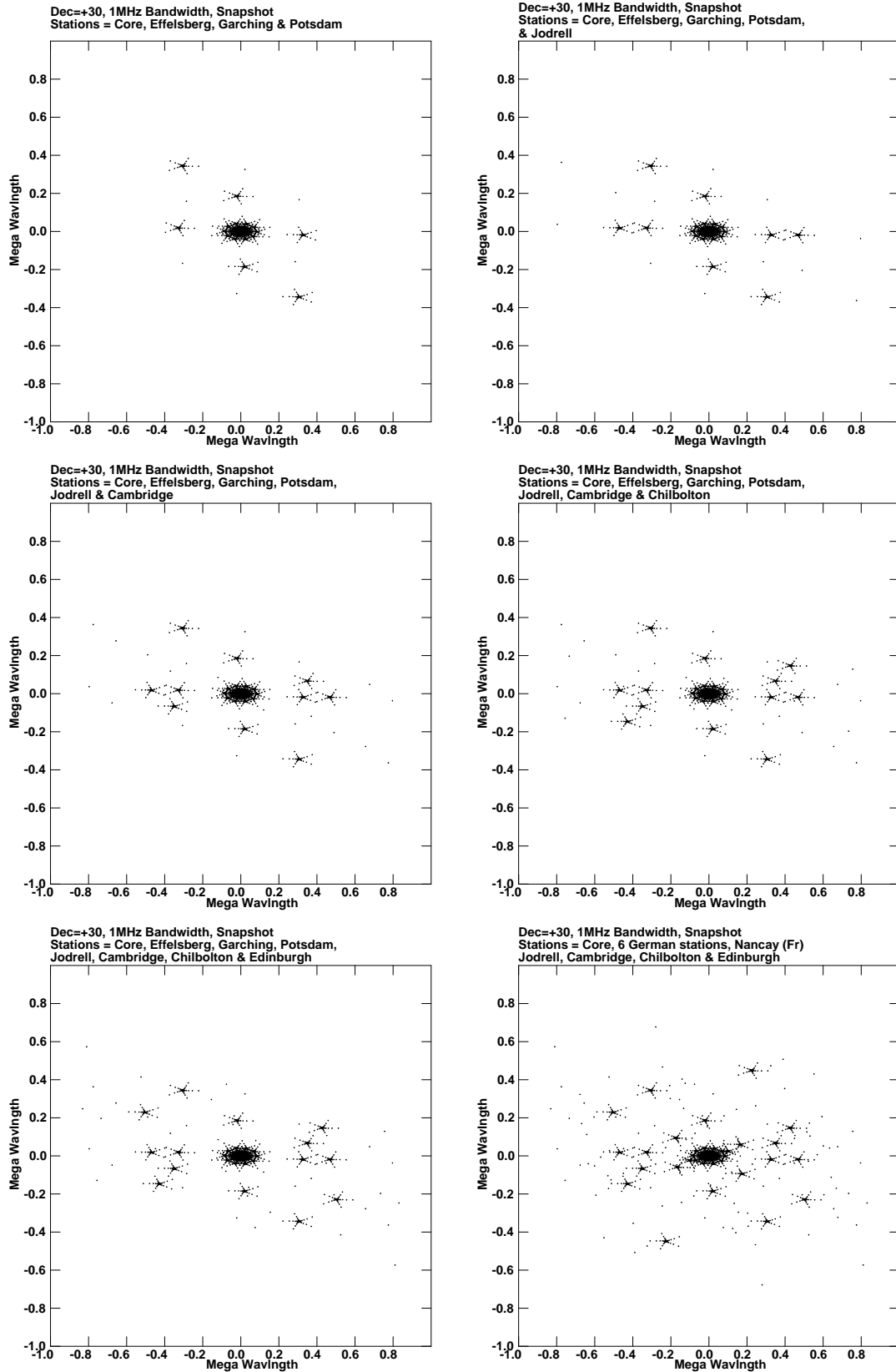
Figure 30: The simulated u-v coverage for snapshot observations at 230 MHz (other frequencies only change the axis scalings), with 1 MHz bandwidth, of a source at 30^\circ declination. The top-left plot shows the u-v coverage provided by the Dutch LOFAR plus three fully-funded German stations. The subsequent four plots show the improvement in u-v coverage when various subsets of UK stations are added. The lower-right plot finally shows the u-v coverage produced from 6 German, 1 French and 4 UK stations.
