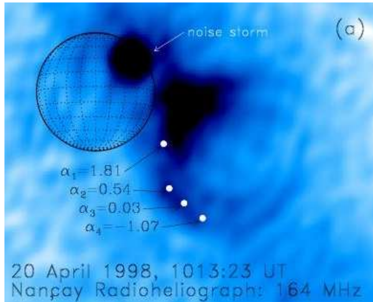
Figure 25: The radio signature of a coronal mass ejection from the Nançay Radioheliograph (Bastian et al., 2001).
