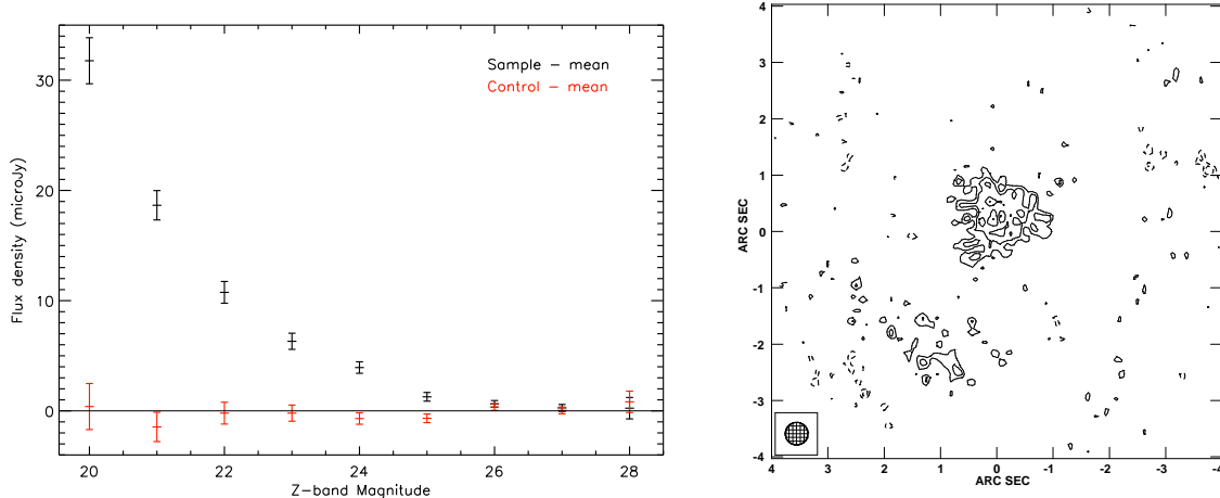
Figure 12: Left: Statistical detection of the \mu\text{Jy} radio emission from >8000 optically selected galaxies within an 8.5 \times 8.5 square arcminute field centred on the HDF-N (excluding all radio emission brighter than 20\mu\text{Jy beam}^{-1} ). Radio emission is statistically detected from galaxies brighter than magnitude 25. The red points represent a control sample of randomly selected positions away from any catalogued source. Right: The average radio emission from 957 galaxies in the HDF-N with magnitudes between 22.5 – 23.5. The contours are \sqrt{2} times 340 \text{ nJy beam}^{-1} .
